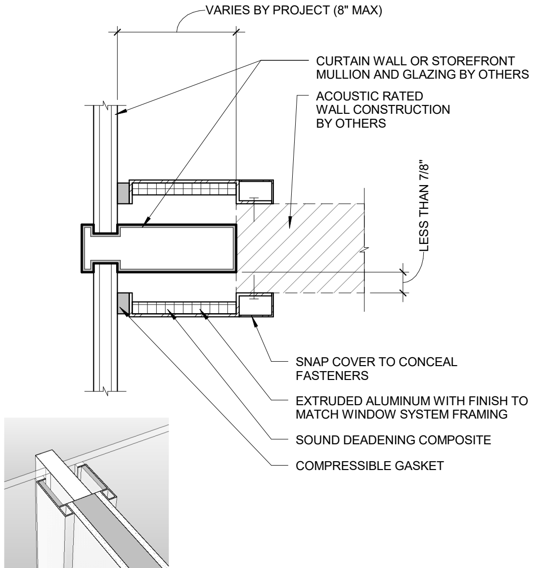
3D VIEW
